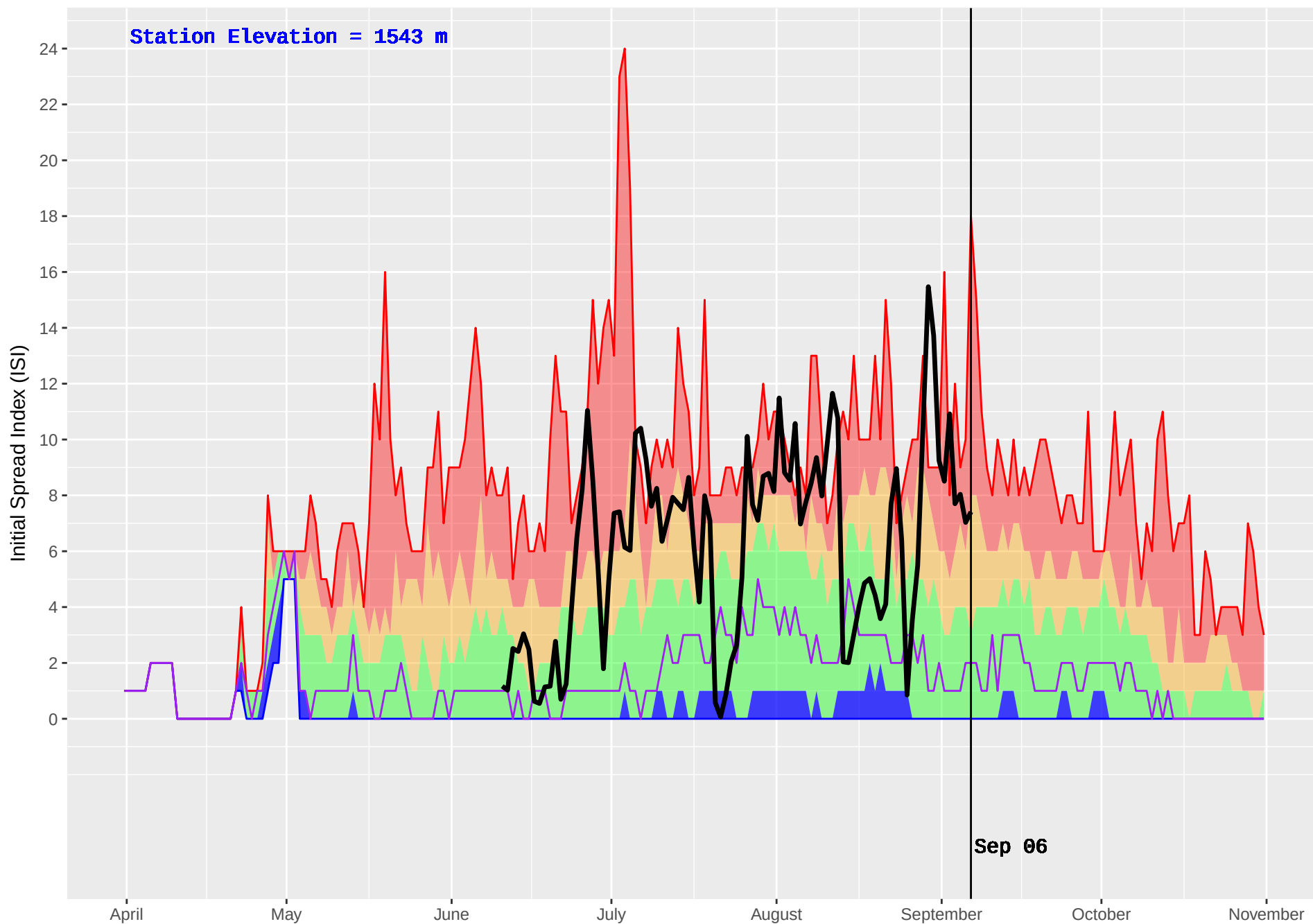
CAHILTY (253) : Historical (1987–2016) and Current (2017) Noon Initial Spread Index (ISI)
