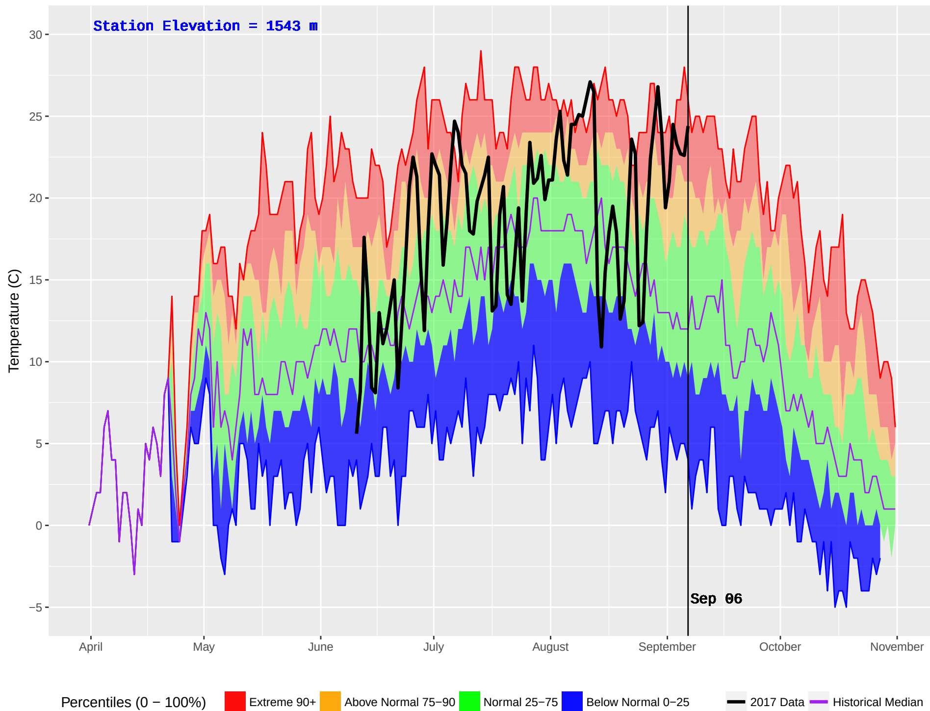
CAHILTY (253) : Historical (1987–2016) and Current (2017) Noon Temperature
