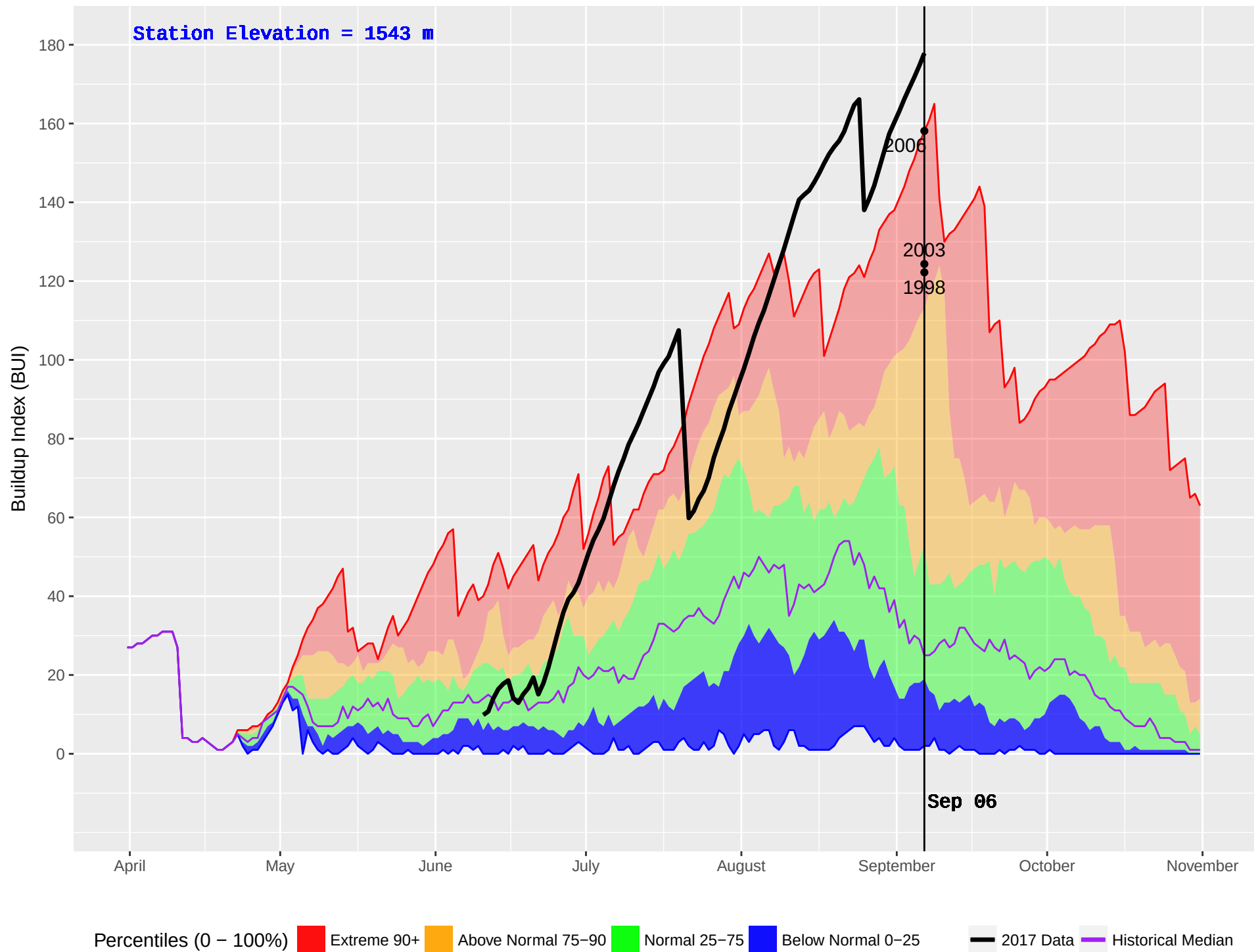
CAHILTY (253) : Historical (1987–2016) and Current (2017) Noon Buildup Index (BUI)
